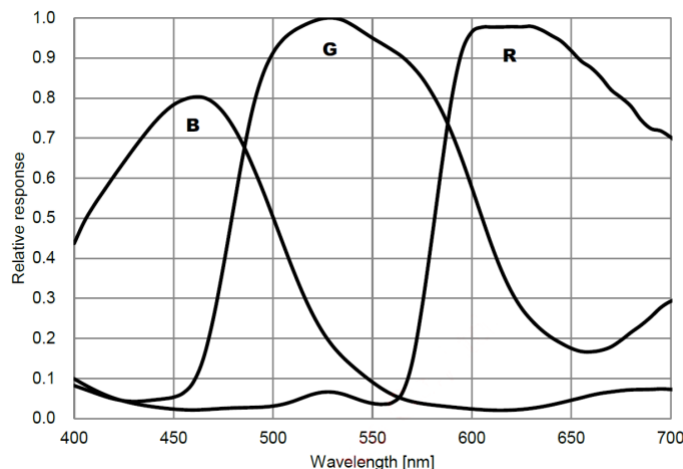
Figure 2 IMX294 Spectral Sensitivity Characteristic
