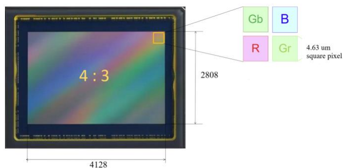
Figure 1 IMX294 Sensor and Its Pixel Structure
