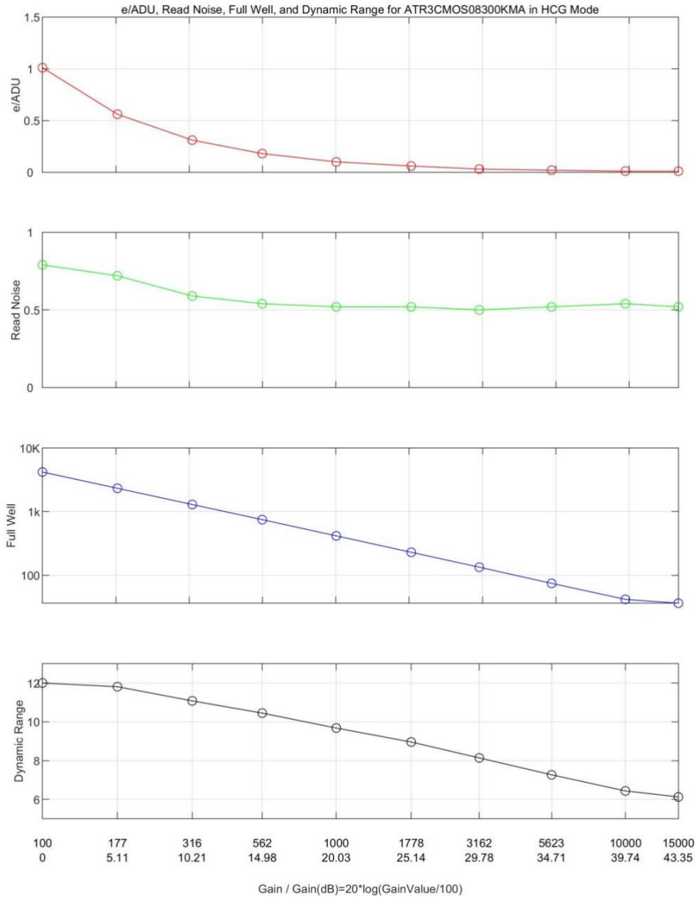
Figure 5 e-/ADU, Read Noise, Full Well and Dynamic Range for ATR585M
