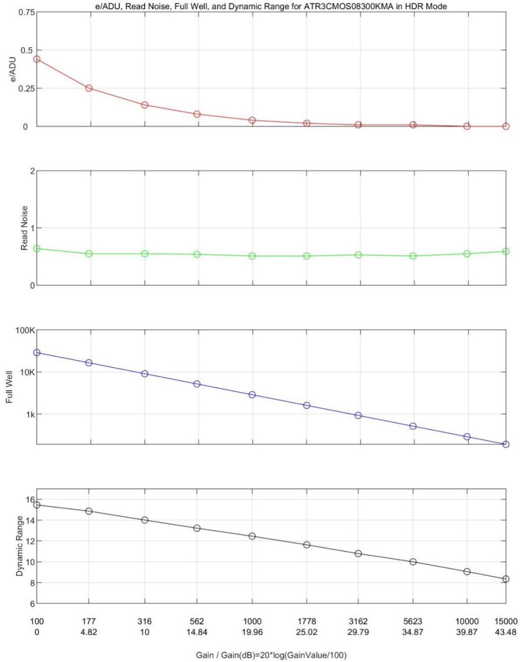
Figure 7 e-/ADU, Read Noise, Full Well and Dynamic Range for ATR585M
