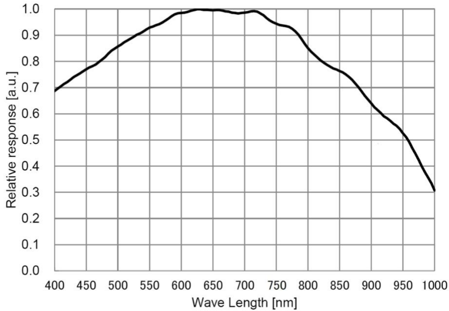
Figure 2 IMX585 Spectral Sensitivity Characteristic
