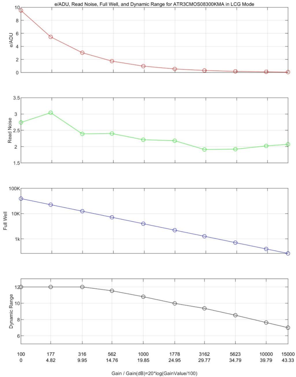
Figure 6 e-/ADU, Read Noise, Full Well and Dynamic Range for ATR585M
