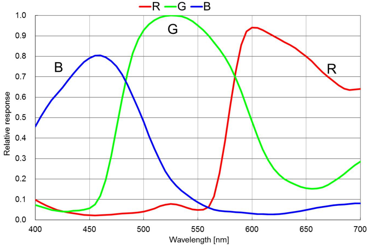
Figure 1 IMX178 Spectral Sensitivity Characteristic
