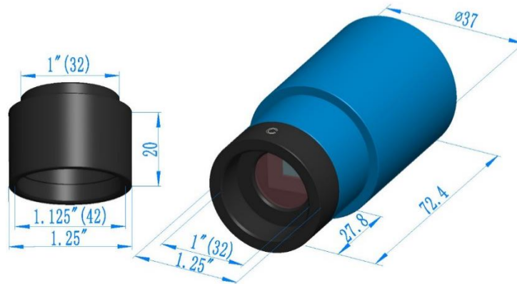
Figure 8 Dimension and Mount of G3M178C and 1.25" extender
