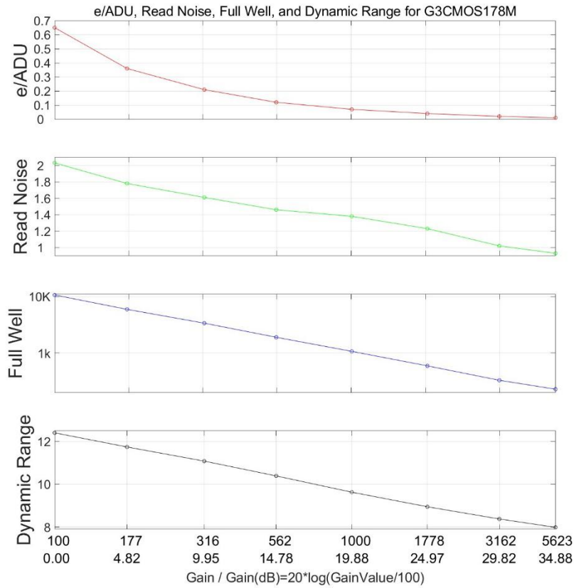
Figure 4 e-/ADU, Read Noise, Full Well and Dynamic Range for G3M178M
