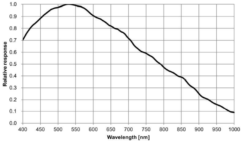
Figure 1 IMX178 Spectral Sensitivity Characteristic
