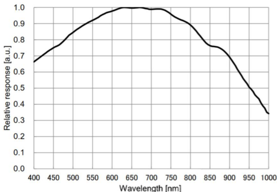
Figure 1 IMX662 Spectral Sensitivity Characteristic
