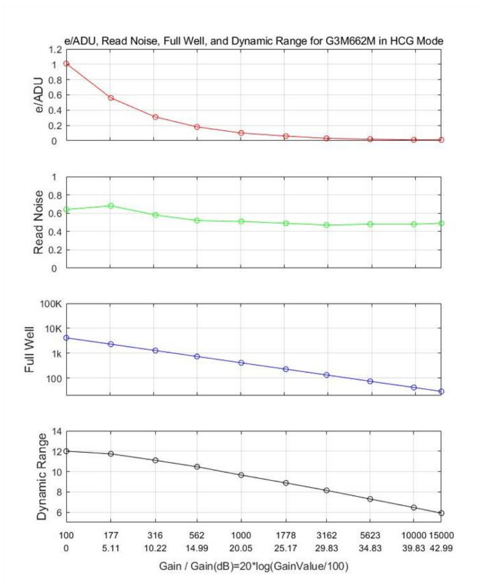
Figure 3 e-/ADU, Read Noise, Full Well and Dynamic Range for G3M662M
