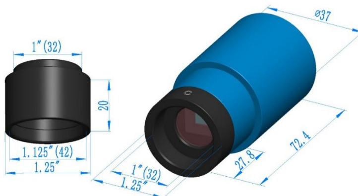
Figure 6 Dimension and Mount of G3M662M and 1.25" extender
