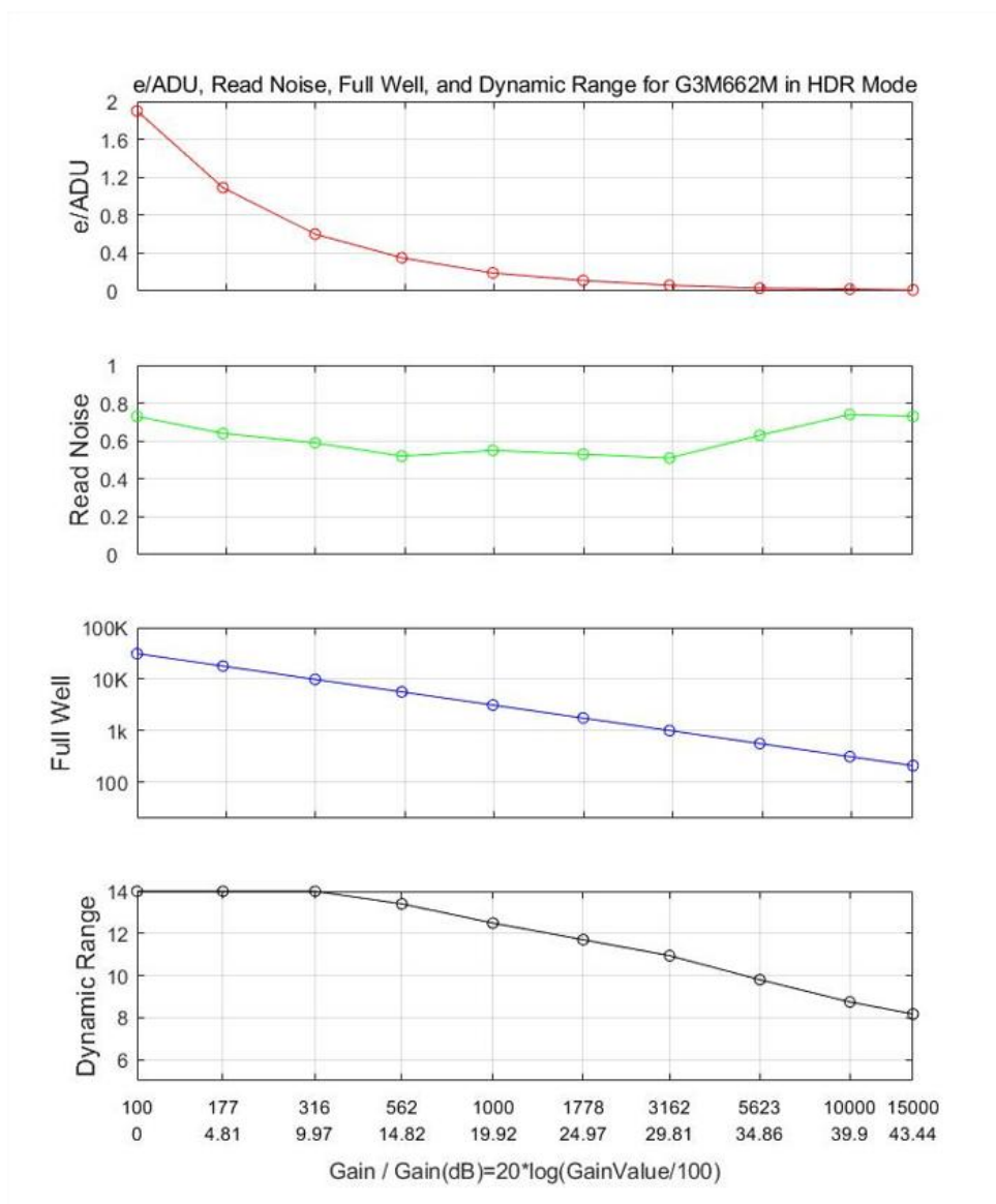
Figure 4 e-/ADU, Read Noise, Full Well and Dynamic Range for G3M662M
