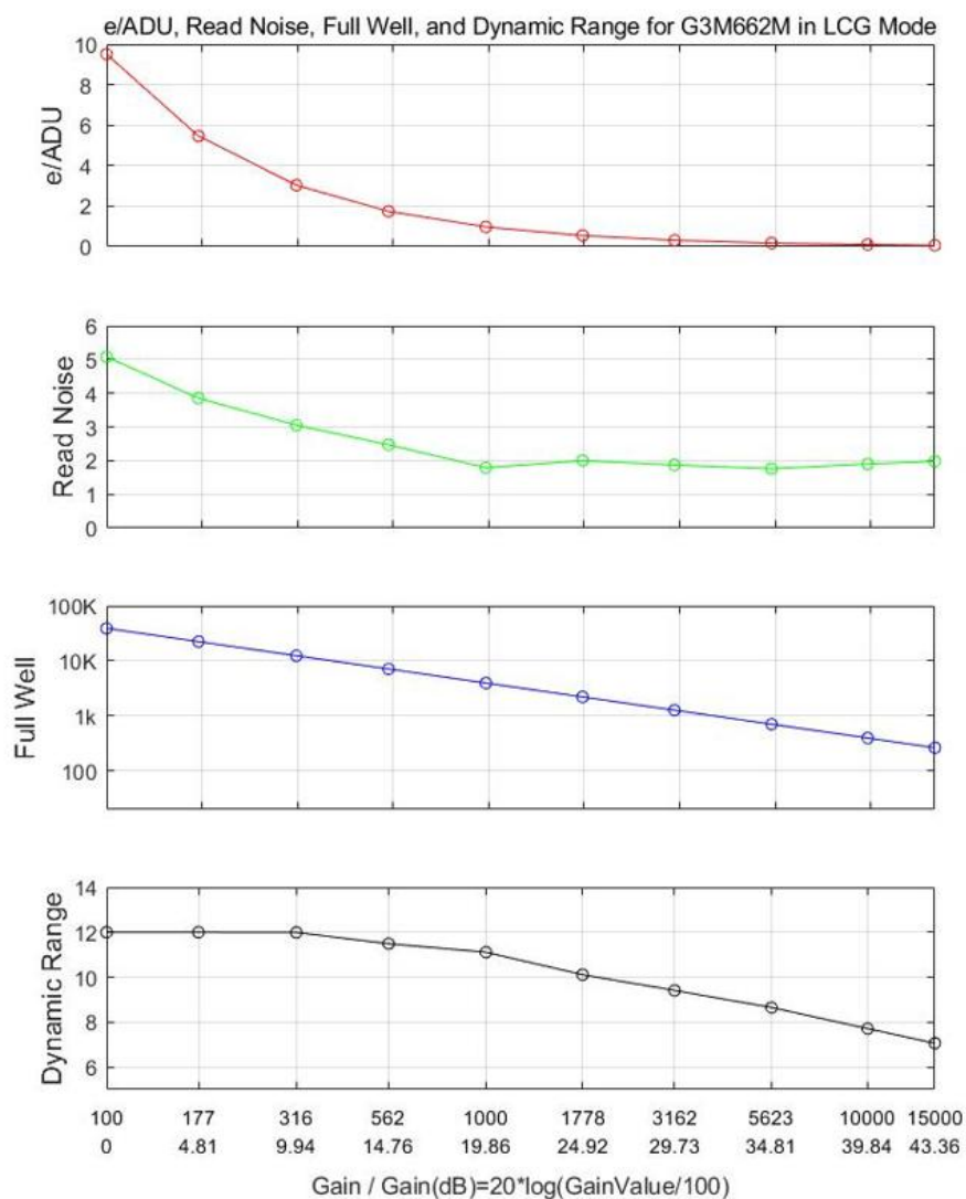
Figure 2 e-/ADU, Read Noise, Full Well and Dynamic Range for G3M662M
