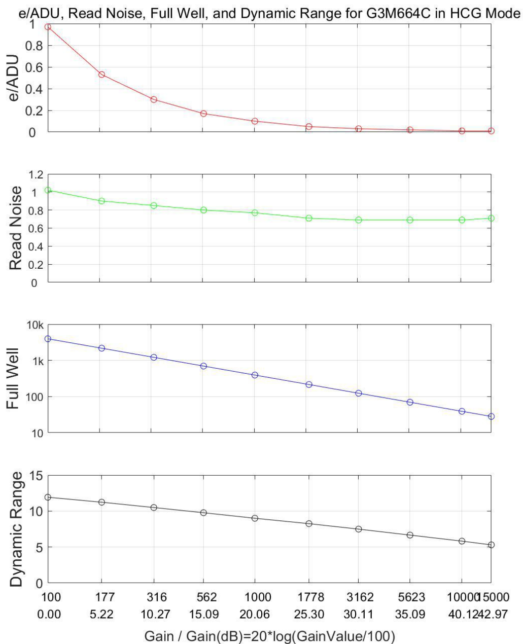
Figure 4 e/ADU, Read Noise, Full Well and Dynamic Range for G3M664C
