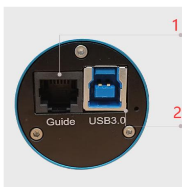
Figure 8 Camera Outline and Interface.
