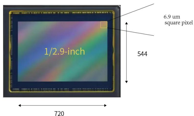
Figure 1 IMX664 Sensor and Its Pixel Structure
