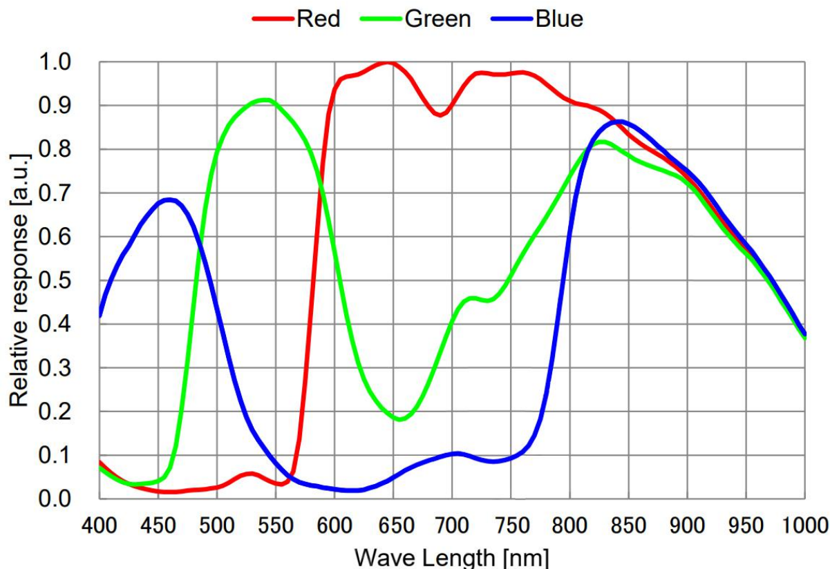
Figure 2 IMX664 Spectral Sensitivity Characteristic
