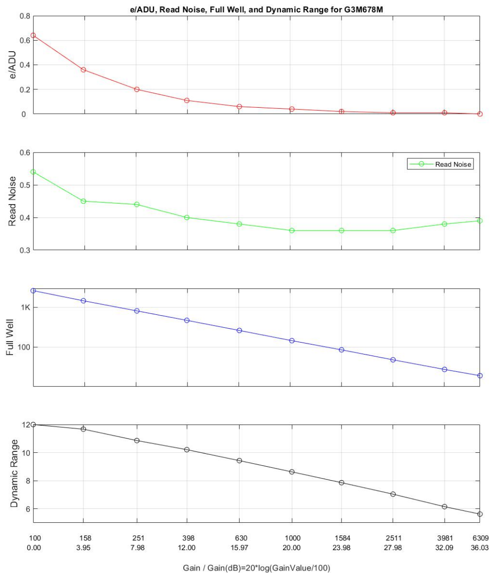
Figure 5 e/ADU, Read Noise, Full Well and Dynamic Range for G3M678M
