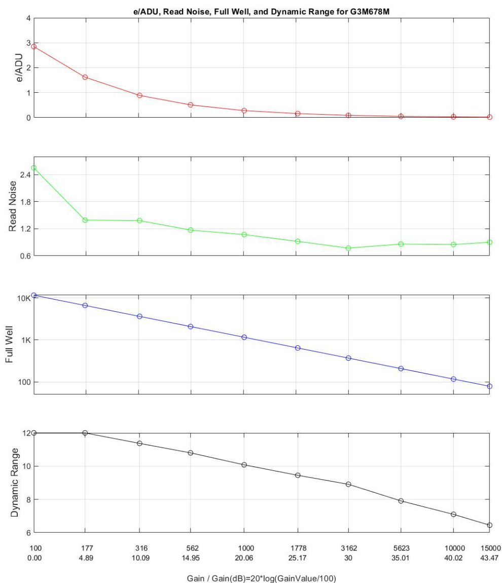
Figure 4 e-/ADU, Read Noise, Full Well and Dynamic Range for G3M678M
