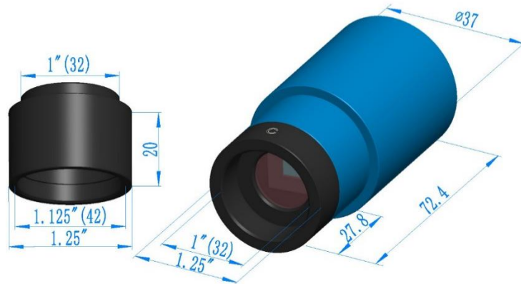
Figure 8 Dimension and Mount of G3M678M and 1.25 inch extender
