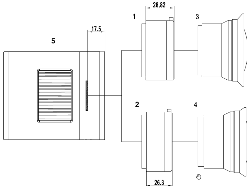
Figure 11 Nikon /Canon Lens with SkyEye Camera
