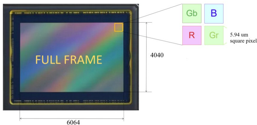
Figure 1 IMX410 Sensor and Its Pixel Structure
