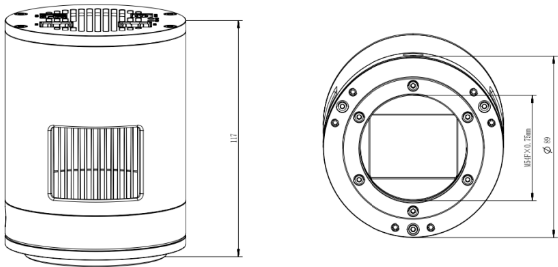
Figure 8 Dimension and Mount of SkyEye24AC-plus
