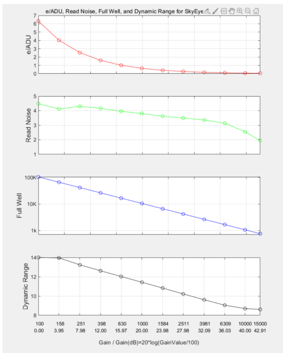
Figure 6 e-/ADU, Read Noise, Full Well and Dynamic Range for SkyEye24AC-plus
