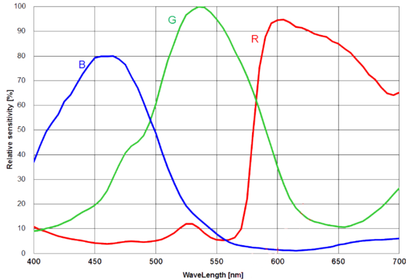
Figure 2 IMX410 Spectral Sensitivity Characteristic
