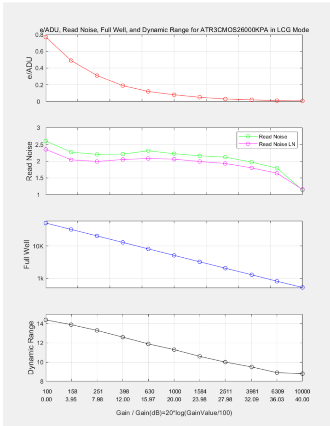
Figure 6 e/ADU, Read Noise, Full Well and Dynamic Range for SkyEye26AC-plus
