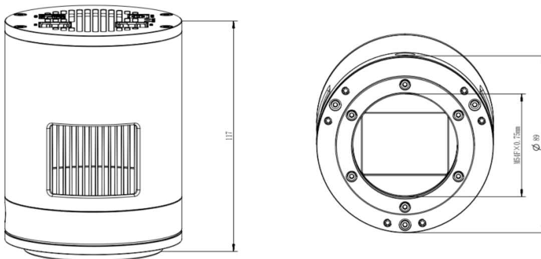
Figure 8 Dimension and Mount of SkyEye26AC-plus
