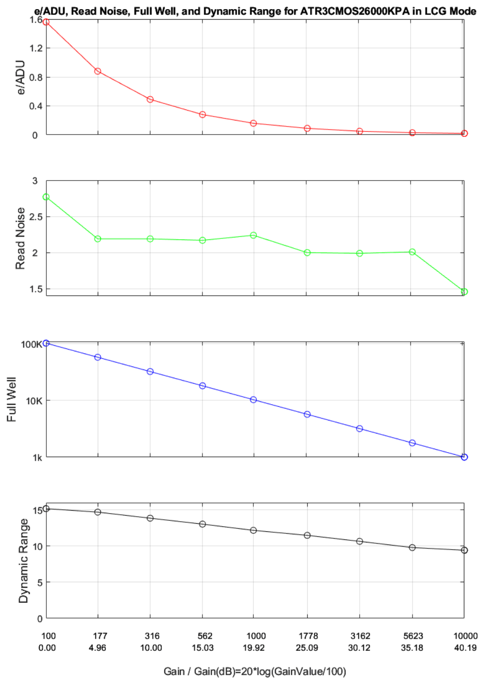
Figure 6.1 e-/ADU, Read Noise, Full Well and Dynamic Range for SkyEye26AC-plus
