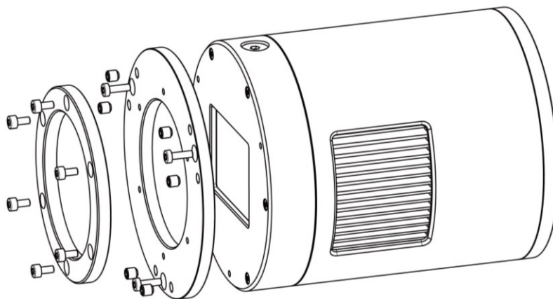
Figure 12 Tilt Adjustment
