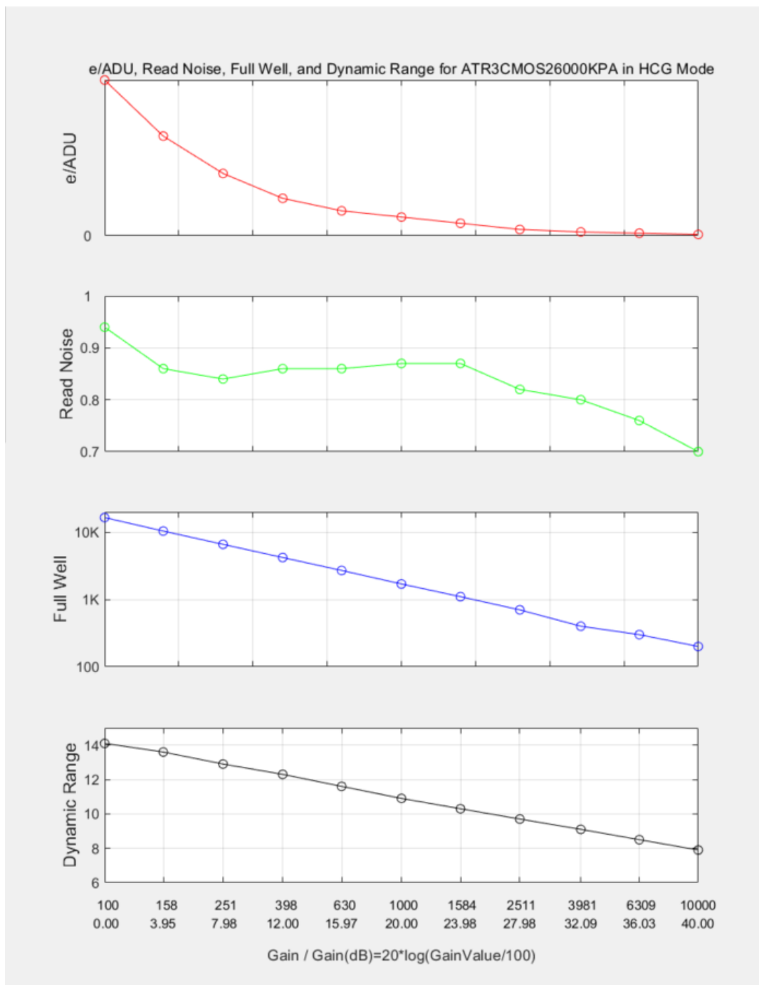
Figure 5 e-/ADU, Read Noise, Full Well and Dynamic Range for SkyEye26AC-plus
