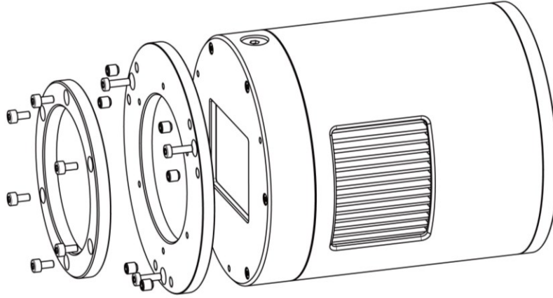
Figure 12 Tilt Adjustment
