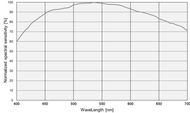
Figure 2 IMX455 Spectral Sensitivity Characteristic
