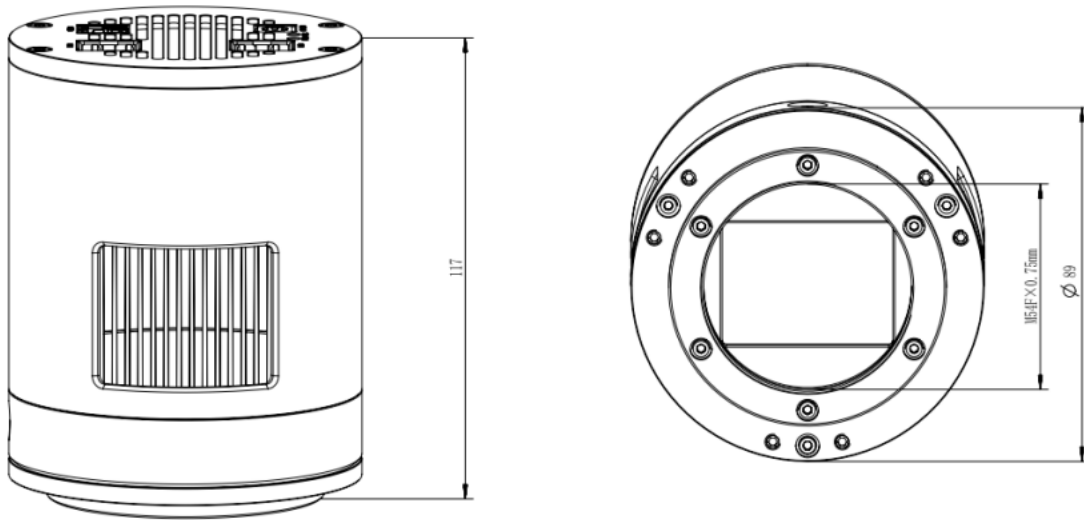
Figure 8 Dimension and Mount of SkyEye62AM-plus
