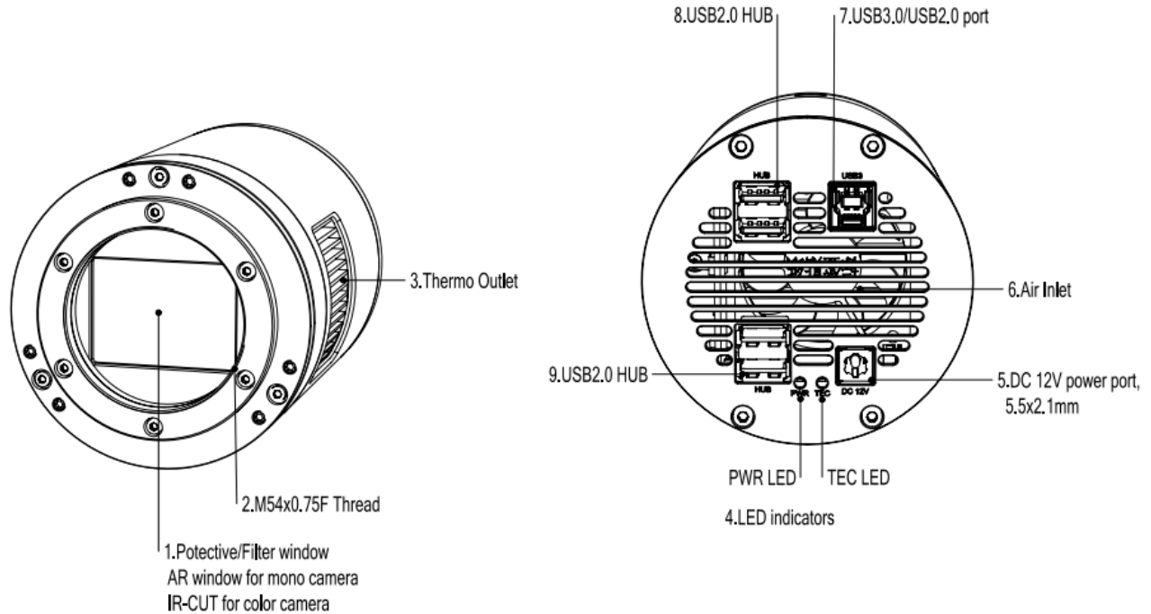
Figure 9 Camera Outline and Interface.
